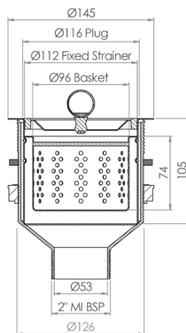
Cross Section
