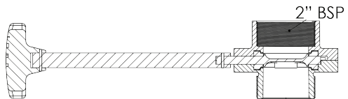
Cross Section
