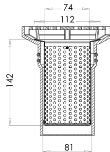
Cross Section
