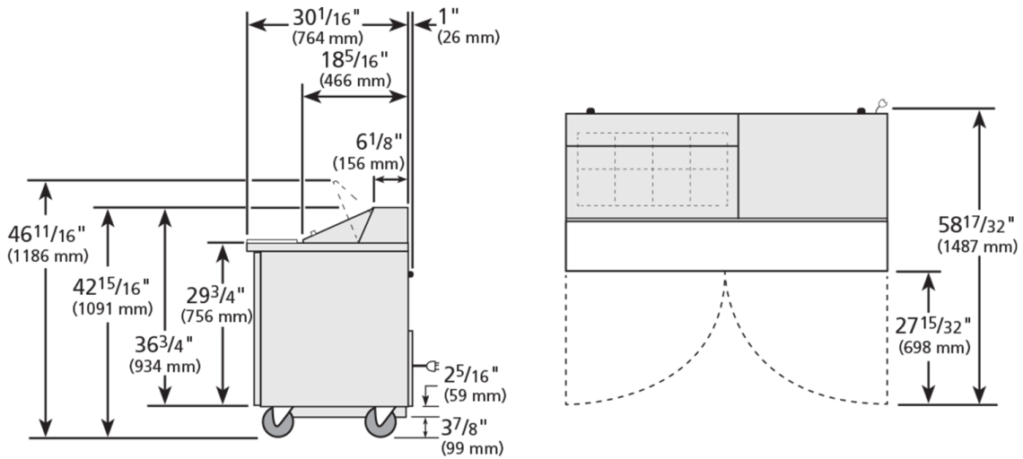
RIGHT VIEW
